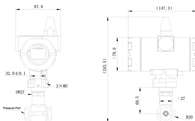
Fig.1 MDM6861 Wireless Differential Pressure
