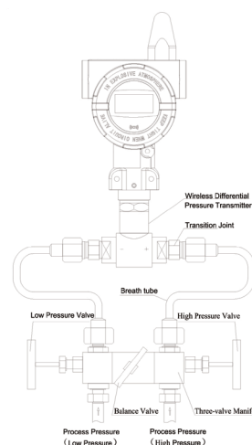
Fig.2 Installation of MDM6861 Wireless Differential Pressure Transmitter
